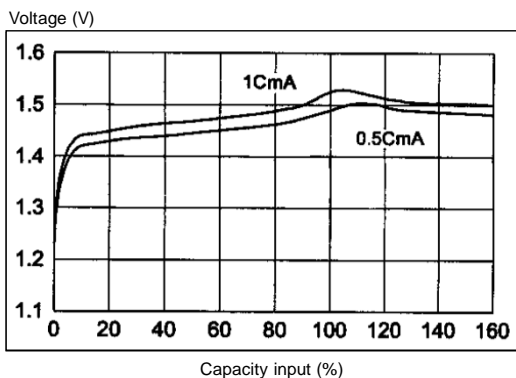
Fast charge curve
