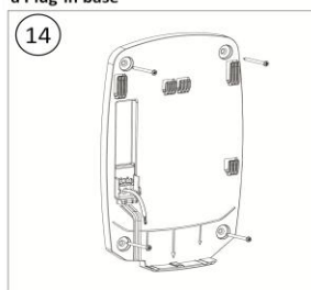
Screw the Plug-in base to the wall (x4)
