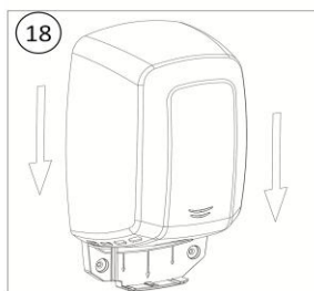
Mount the dryer over the Plug-in base with a from top to down movement
