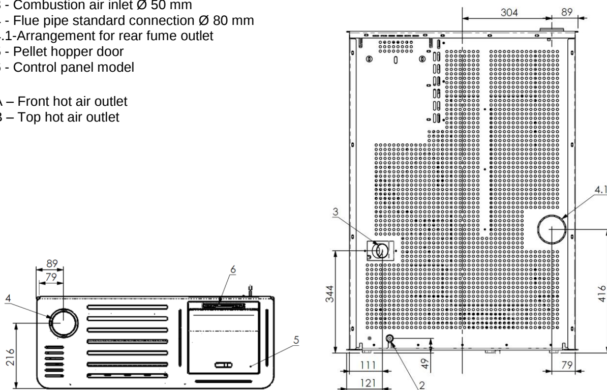
AITANA pellet stove dimensions
