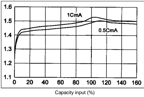
Fast charge curve
