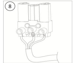
At the back of the unit, connect the wires to the fast connector following the engraved letters (N, L and Earth)
